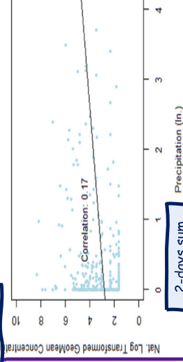
GAL034 2 Day Rainfall Correlation
