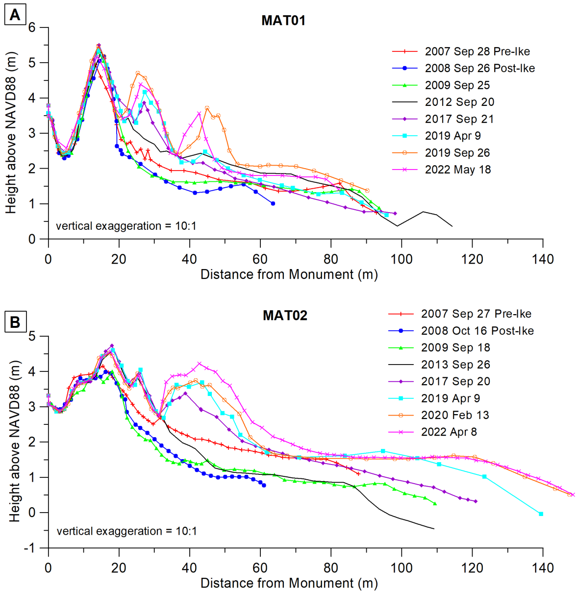
Figure 23. Pre- and post-Hurricane Ike profile data collected by Van Vleck High School students at (A) MAT01 and Palacios High School students at (B) MAT02. Students are monitoring recovery and growth of the foredune at these sites.
