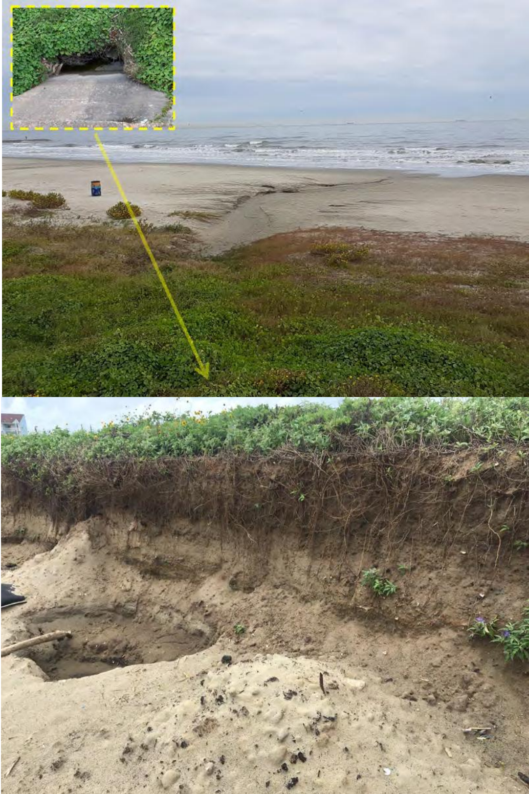
Figure 3. Photos of a runoff scour channel at the seaside toe of the Galveston Seawall (top) and a runoff scour hole at the base of the dune scarp at the Central Beach site. Photos by Youn-Kyung Song (top, date: 03-22/2021) and Jacob Garret (bottom, date: 07-08-2021).
