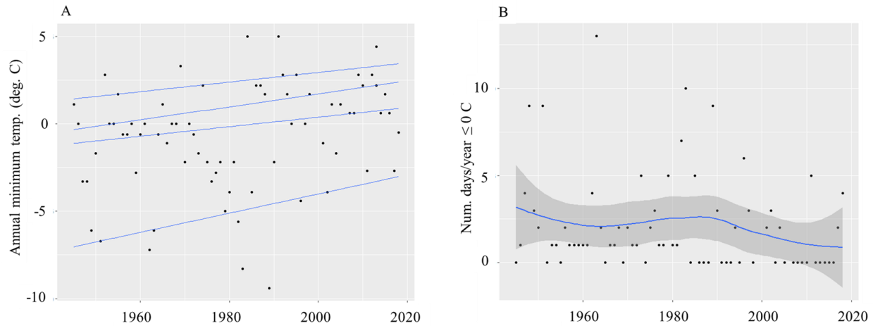
Figure 9. Temperatures from the Naval Air Station in Corpus Christi from 1945 – 2018. A. Quantile regression lines for \tau = 0.1, 0.5, 0.7 , and 0.9 are shown top to bottom respectively. Quantile regression was significant although slopes of the lines were not different from one another indicating that the one for \tau = .5 (simple linear regression) suffices to indicate the pattern of increasing minimum temperatures over time. B. the loess pattern of number of days at or below freezing show a decreasing trend.
