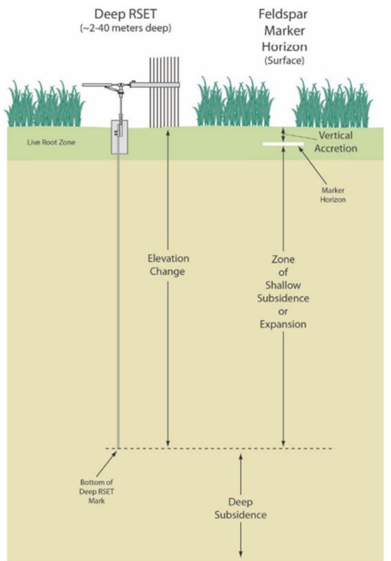
Figure 2. Diagram of deep rod SET and marker horizon from Lynch et al. (2015). The SET measures elevation change relative to the bottom of the steel rod benchmark and the MH (often feldspar) measures vertical accretion. SET minus MH provides a measure of deep subsidence (below the SET rod benchmark).
